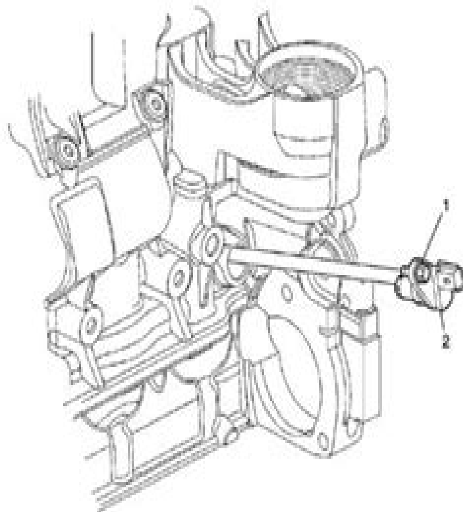
Fig. 97: Crankshaft Position Sensor Courtesy of GENERAL MOTORS CORP.
