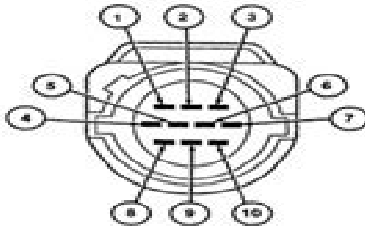
Transaxle Connector/Harness Diagram
