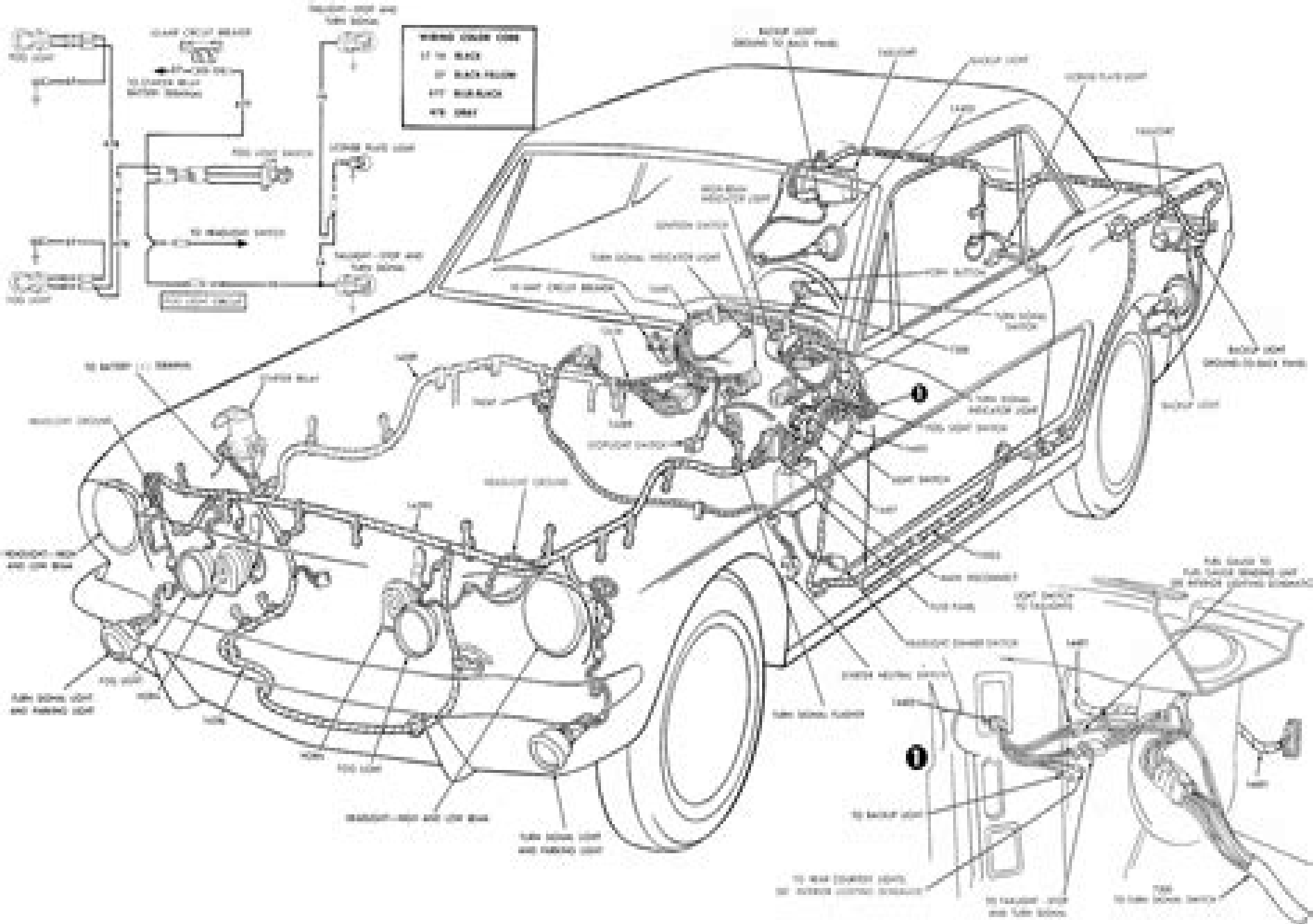
1966 MUSTANG EXTERIOR LIGHTING, TURN SIGNALS AND HORNS
