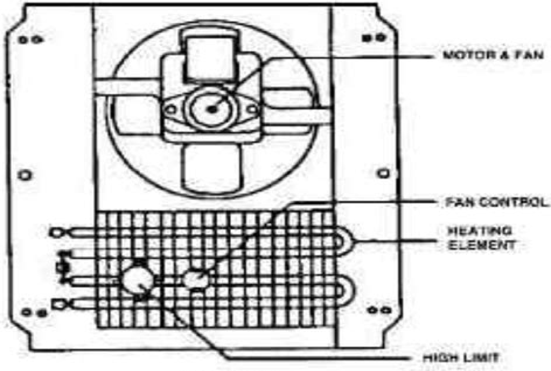
INNER FRAME ASSEMBLY (Back View)
