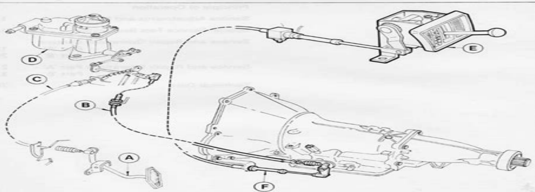
Fig. 1. Automatic transmission operating system
