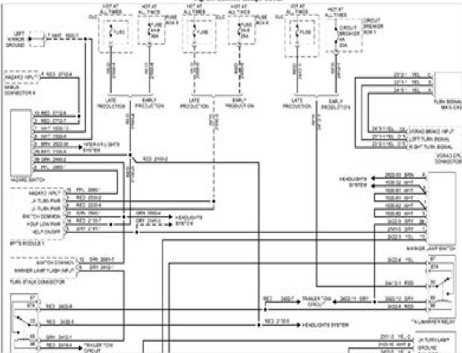
Fig. 28: Exterior Lamps Circuit
