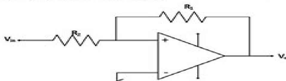
FIG. 7.2 Schmitt Trigger (NONINVERTING MODE)
