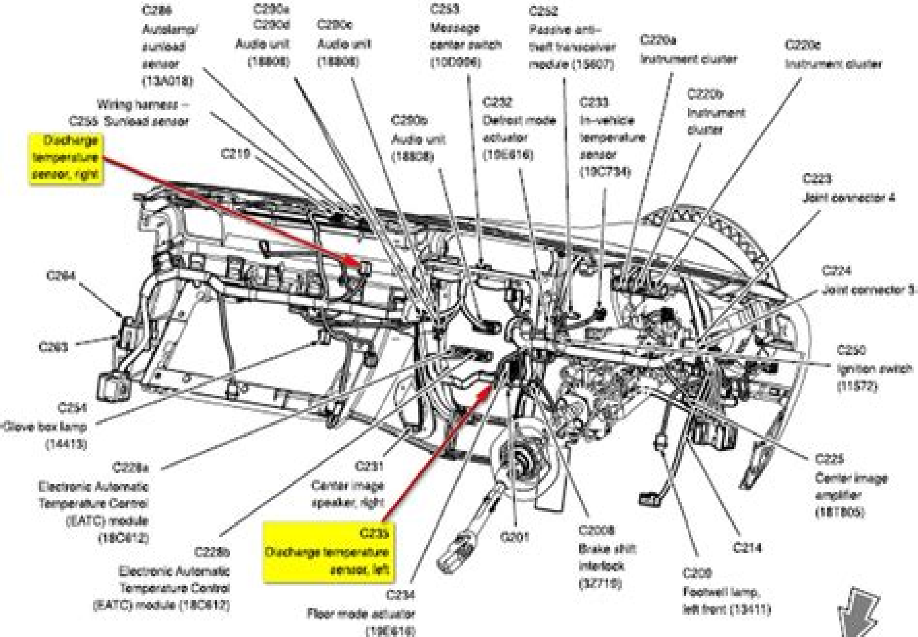
Dash panel – rear view
