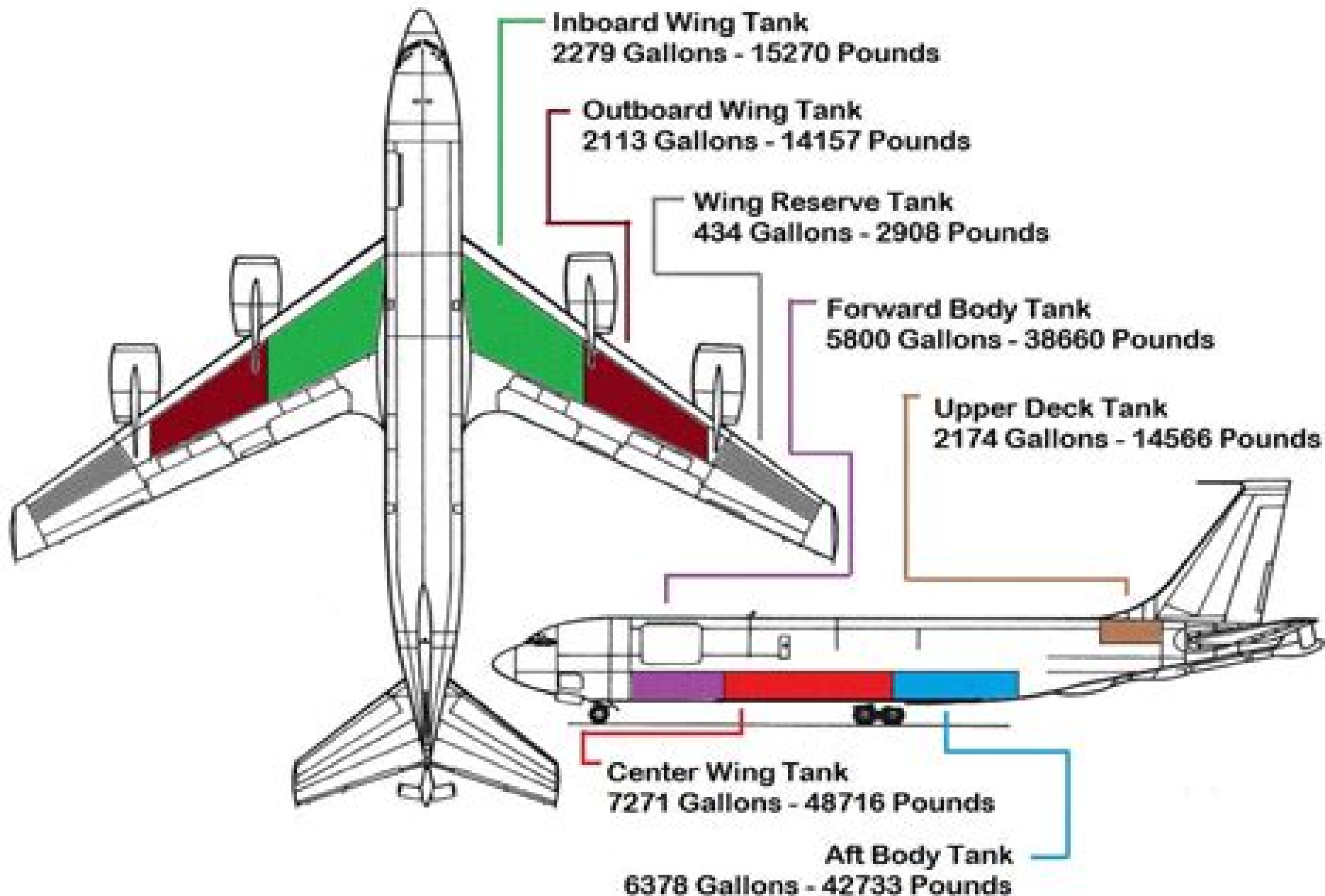
KC-135 Fuel Tank Locations & Quantities
