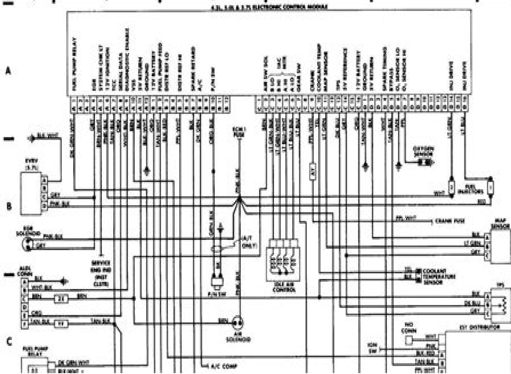
Fig. 2: Engine Compartment (Cont.)
