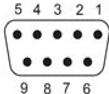
D-Sub 9pin Female
