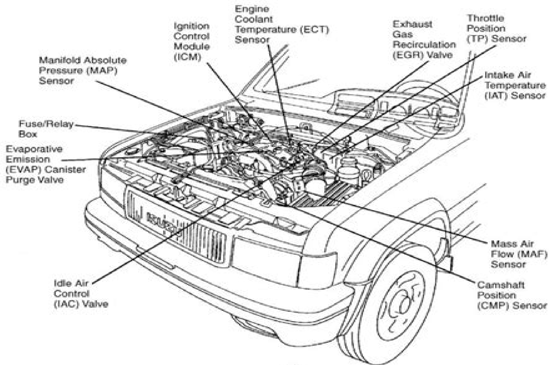
Fig 2: Engine Compartment (3.2L)
