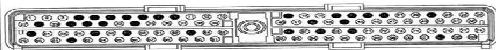
C294 (GRAY) POWERTRAIN CONTROL MODULE (PCM) (4.6L 2V)
