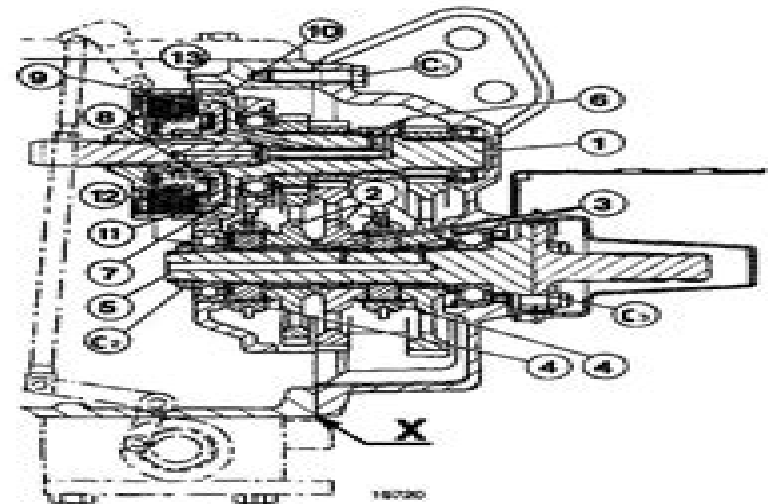
Sectional views of power take-off
