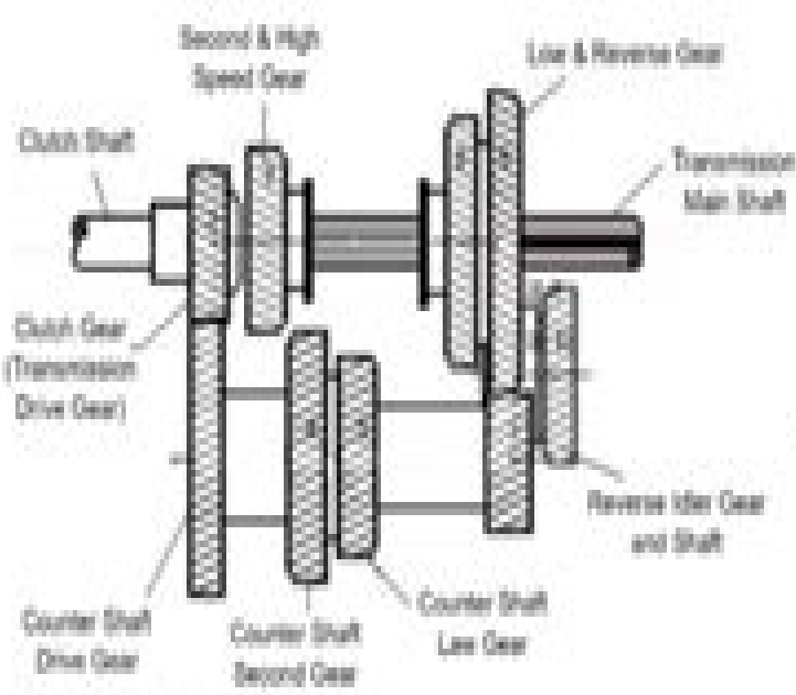
Sliding Mesh Gearbox
