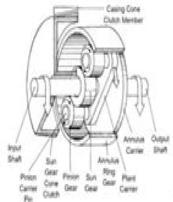
Epicyclic Gearbox
