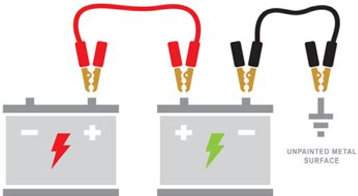
UNCHARGED BATTERY
