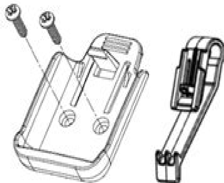
Surface Mount/Belt Clip
