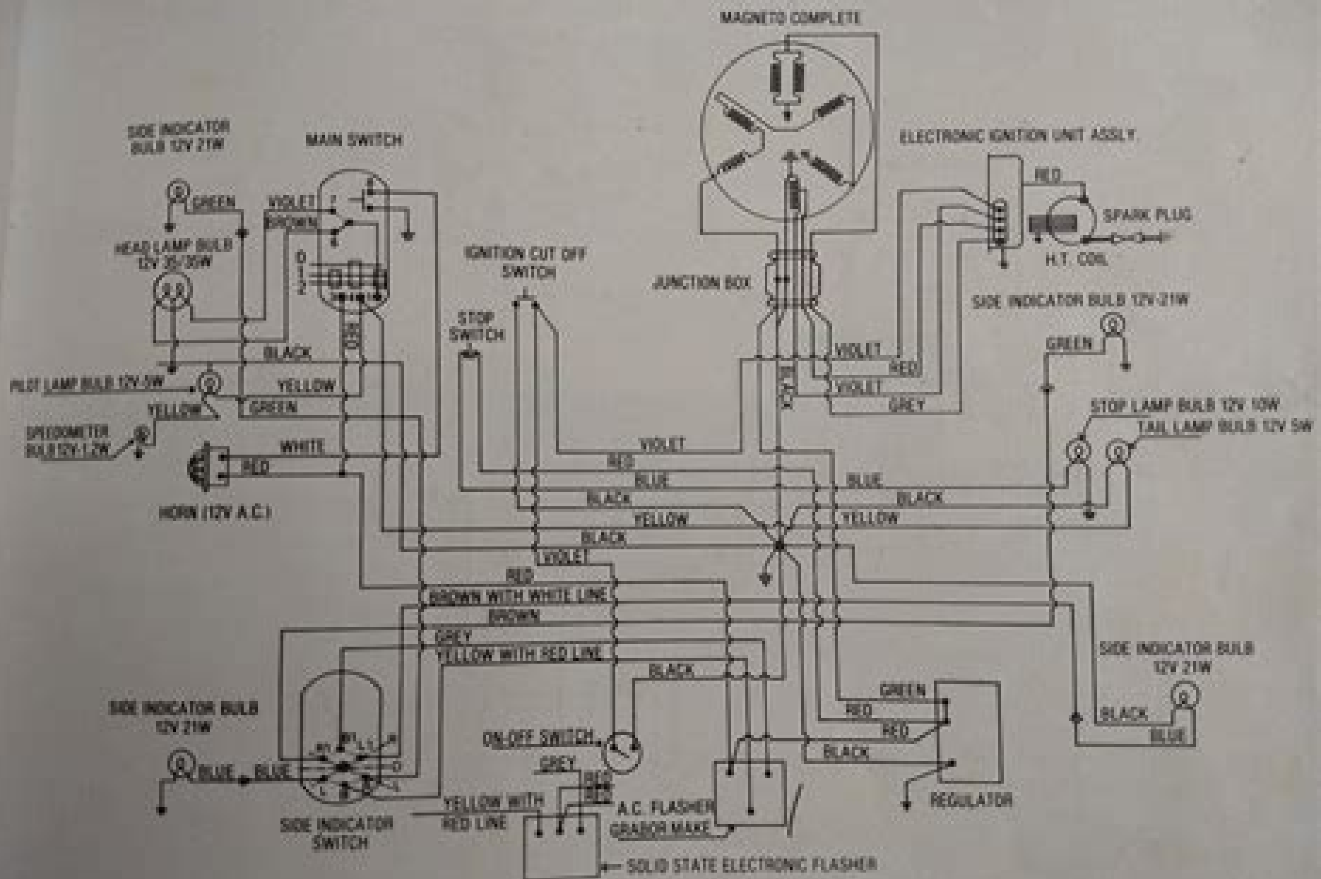
Fig. 21 (g) Wiring diagram for 12V Electronic Ignition System with A. C. Side Indicators.
