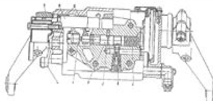
Fig. 15. - Side control shaft section.
