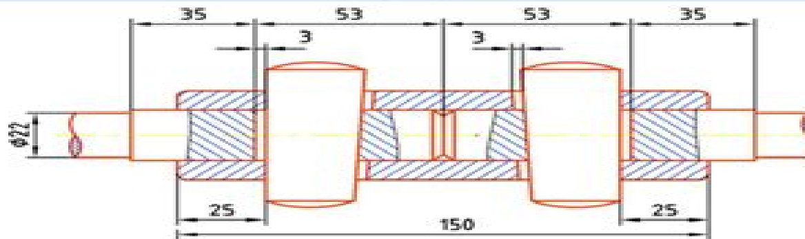
SECTIONAL FRONT VIEW
