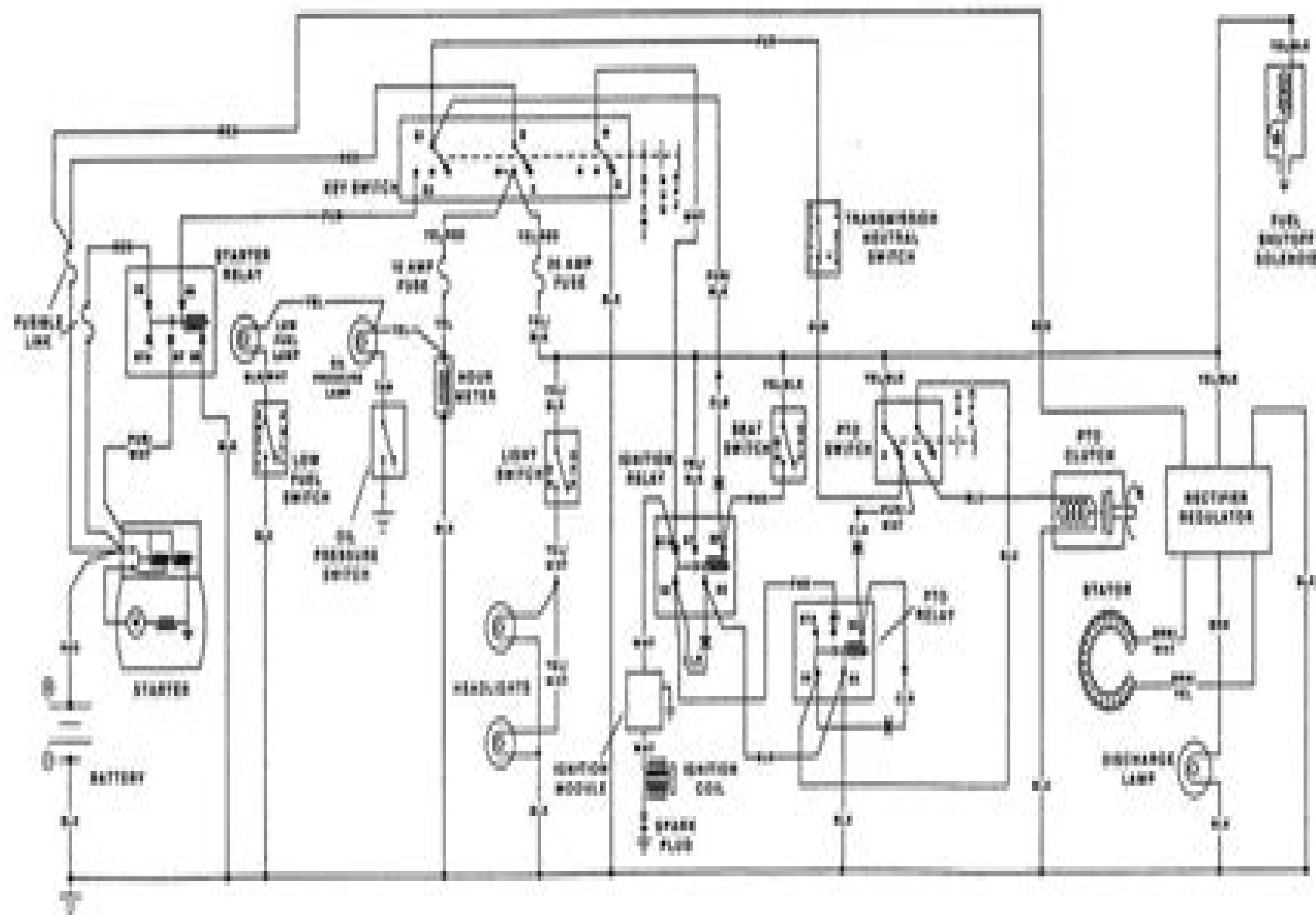
Fig. JD4-20-Electrical system schematic for Models 260 and 265.
