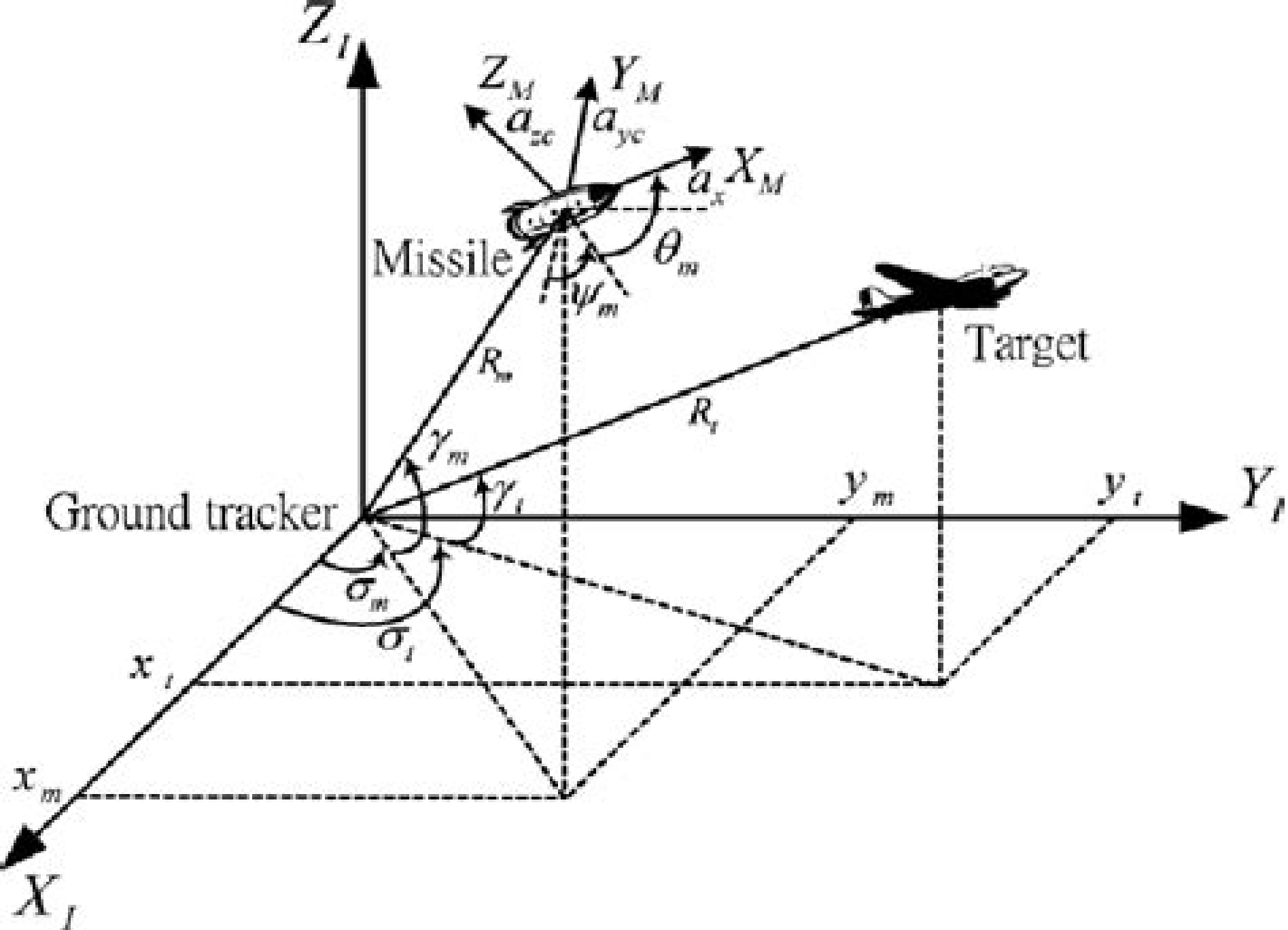
FIG. 1. Diagram of the missile and target tracking in 3-D [13].
