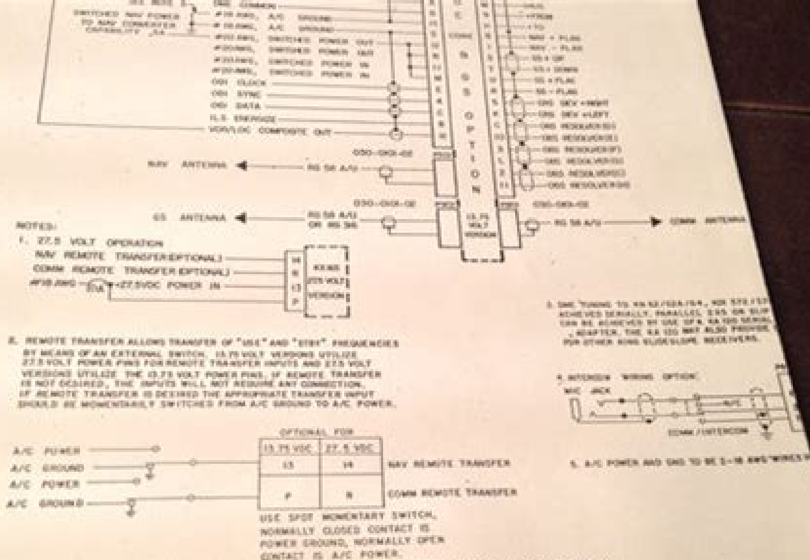
FIGURE 2-6 KX 165 NAV/COMM VOR/LOC CONVERTER W/GS OPTION (Dwg No 155-01345-0000, Rev 4)
