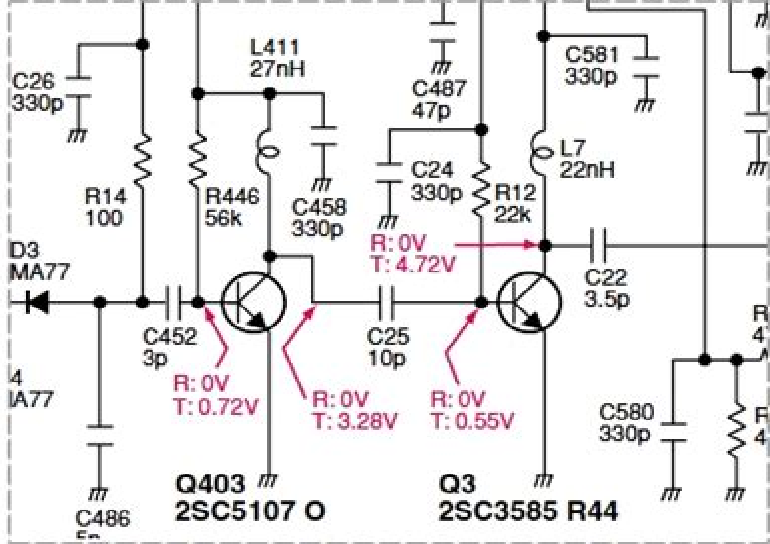
Preview: ICOM IC-F4TR schematic diagram
