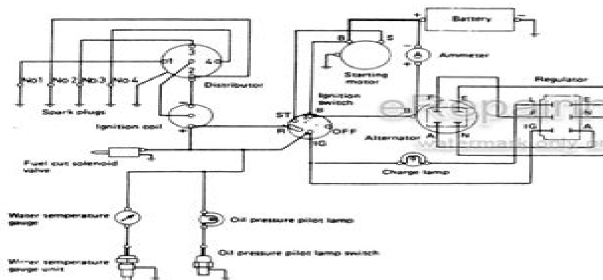
Wiring diagram
