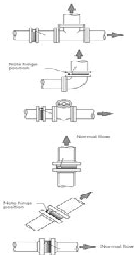
FIGURE 1. Installation positions, elevation view
