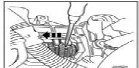
4.8c Using a screwdriver to move the transmission shift forks into neutral
