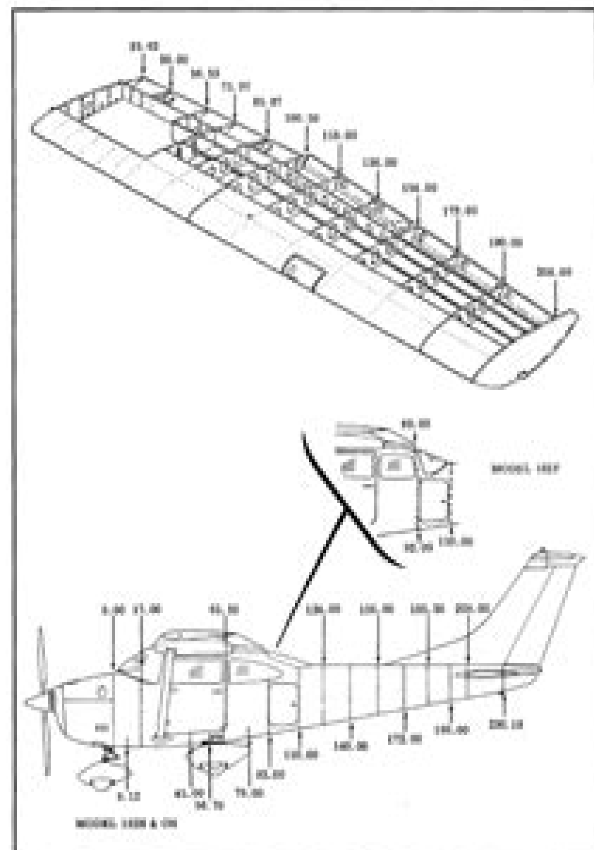
Figure 1-3. Reference Stations - Model 182
