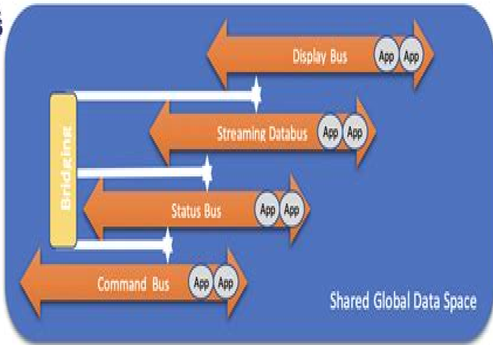
Figure 1. The Layered Databus Architecture
