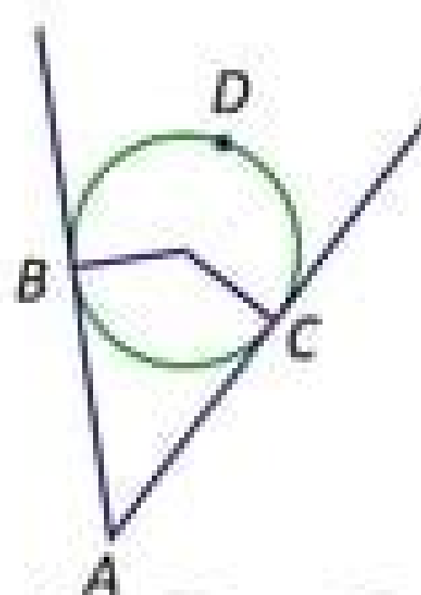
Two Tangents
