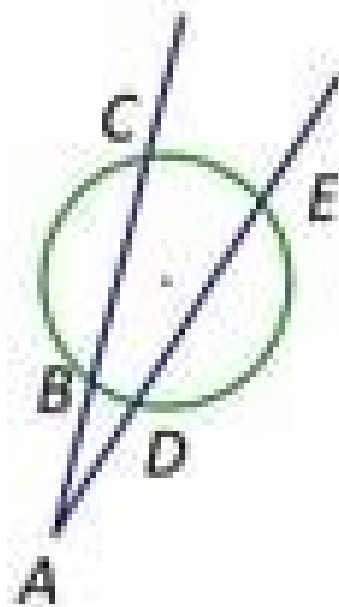
Two Secants
