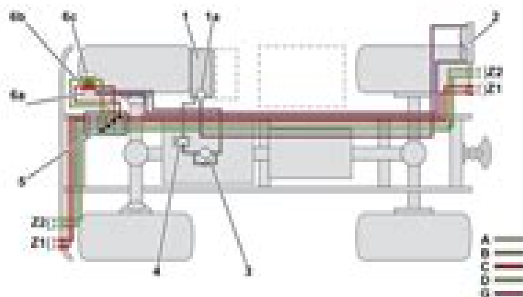
Hydraulic diagram of work hydraulics, front and rear hydraulic system
