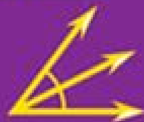
Angle Bisector
