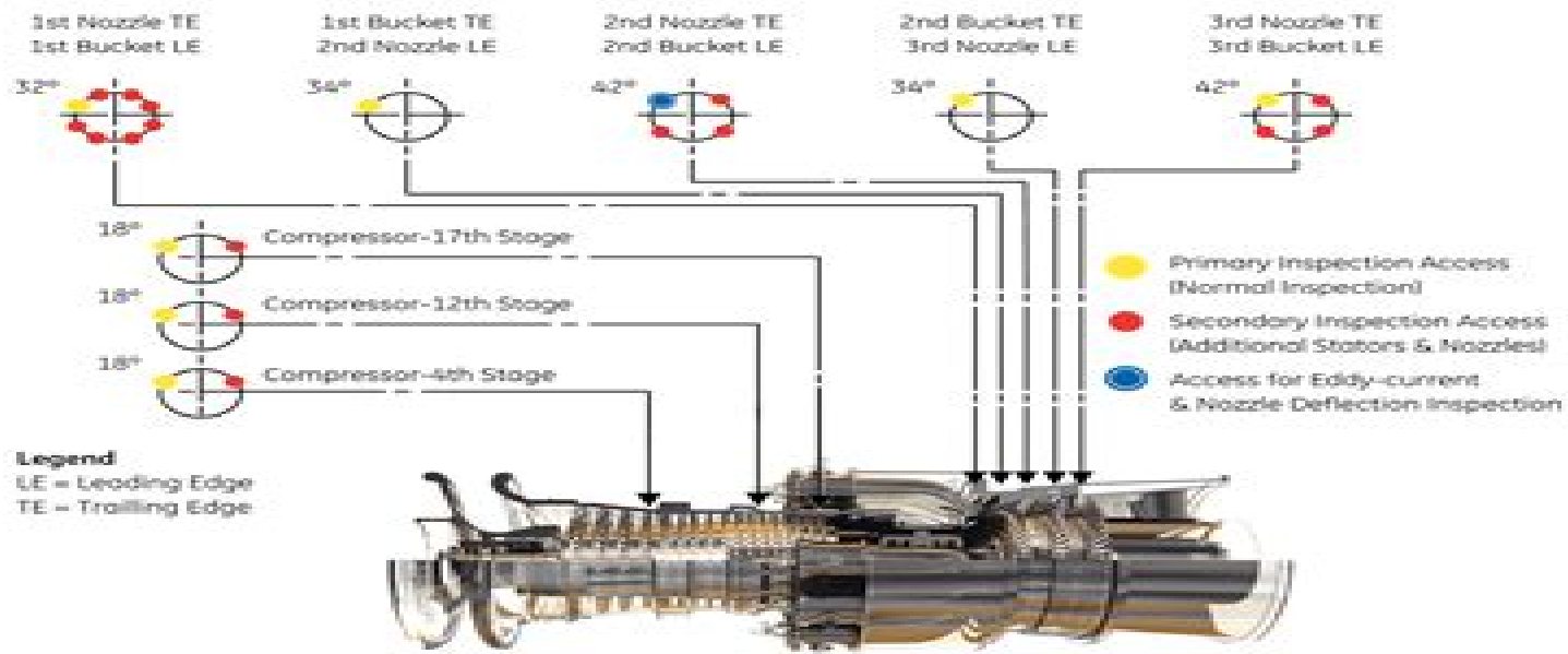
Figure 3. GE D3 gas turbine borescope inspection access locations
