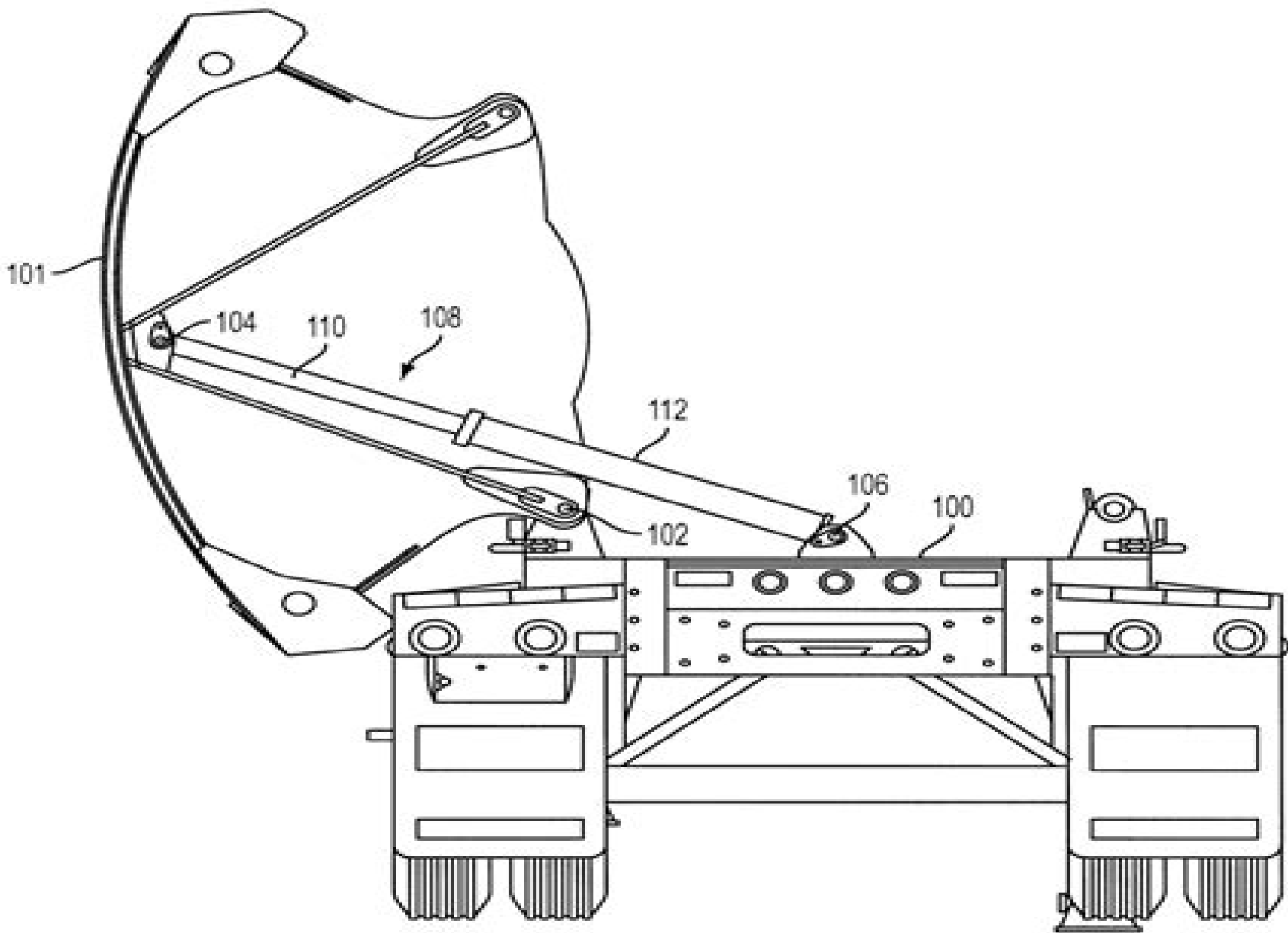
FIG. 4 PRIOR ART
