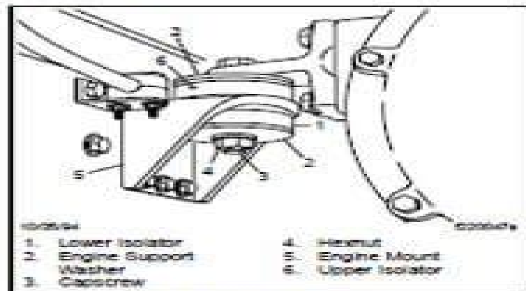
Fig. 1. Rear Engine Mount
