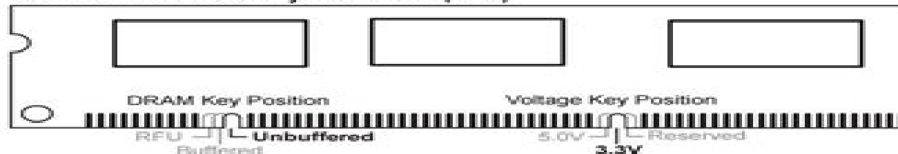
168-Pin DIMM Notch Key Definitions (3.3V)
