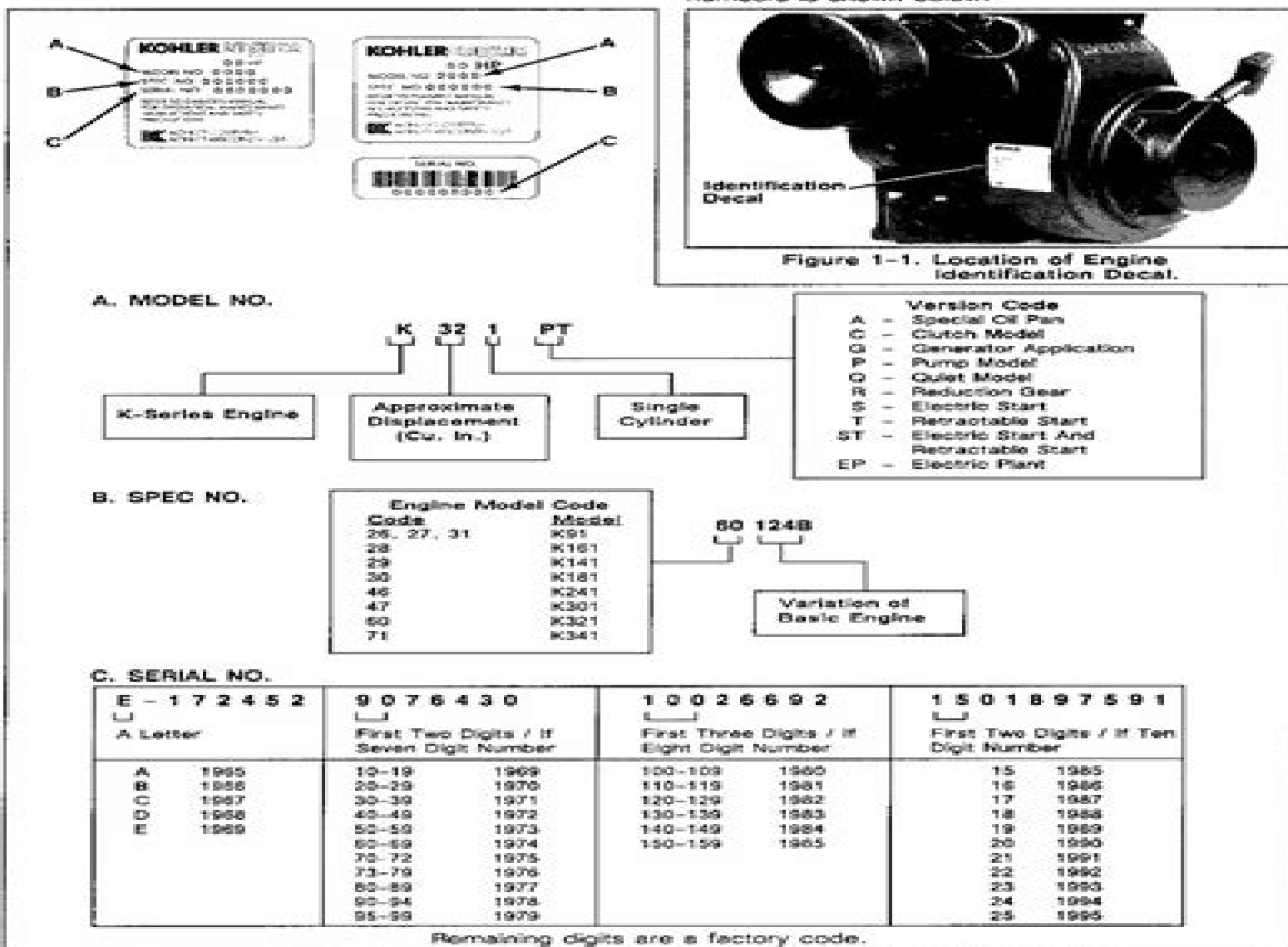
Figure 1-2. Engine Identification Decals.
