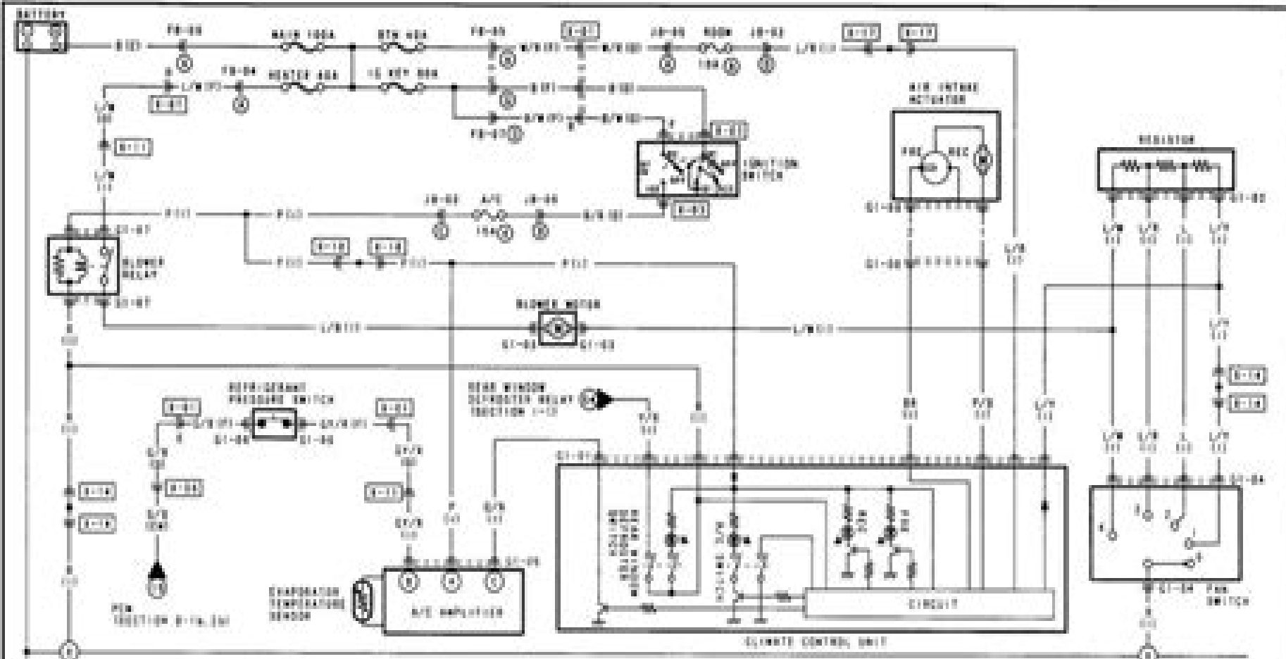
C1-01 CLIMATE CONTROL UNIT
