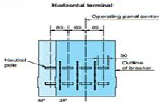
Main circuit terminal dimension
