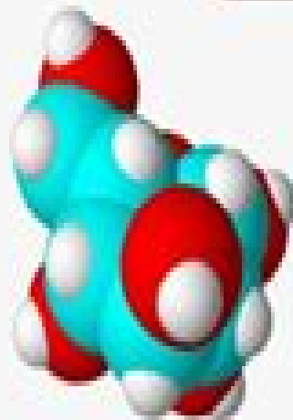
GLUCOSE
