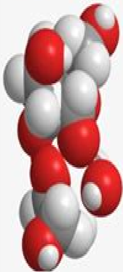
SUCROSE
