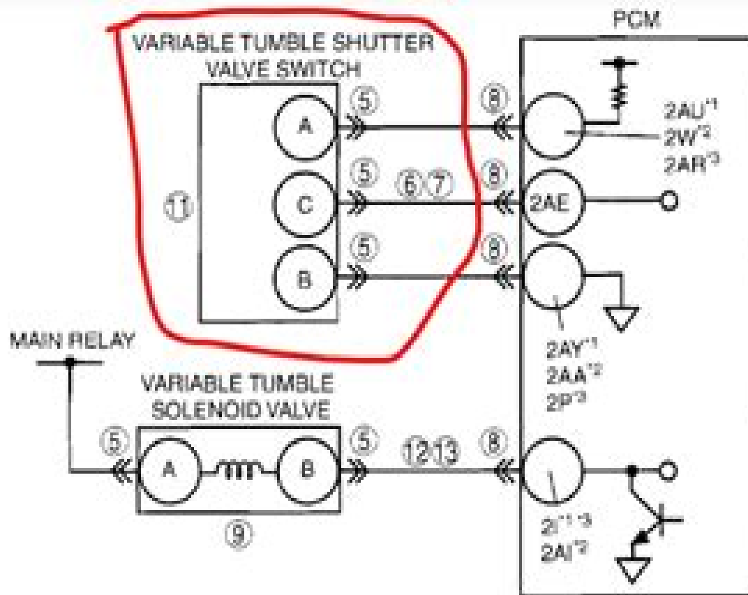
VARIABLE TUMBLE SOLENOID VALVE WIRING HARNESS-SIDE CONNECTOR
