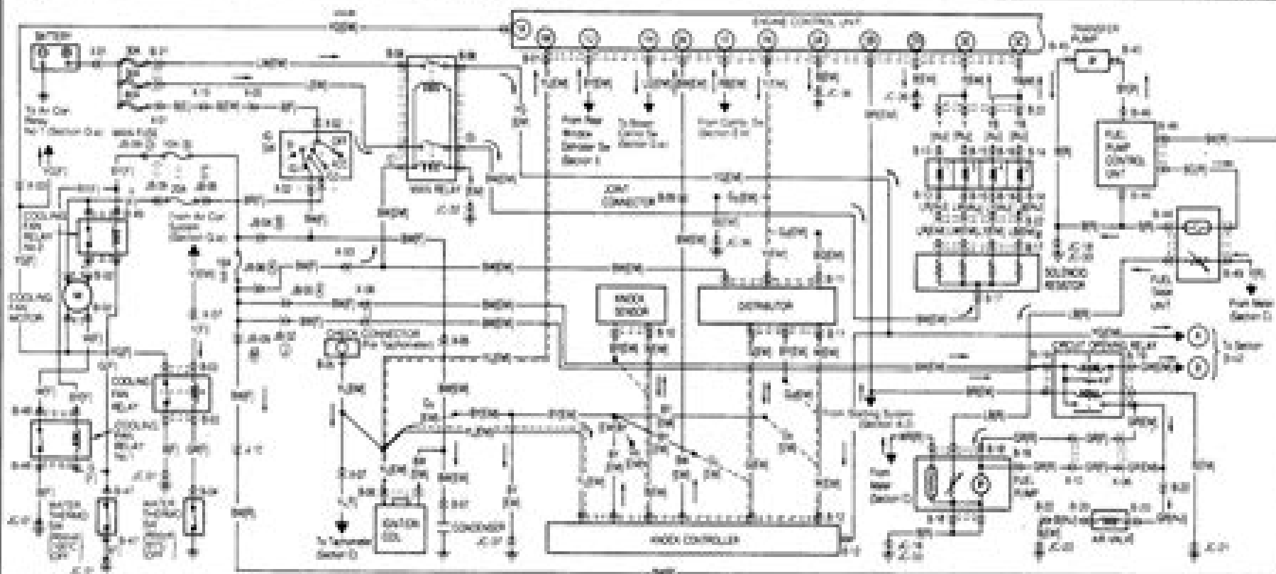
8-17 Engine Control Unit (ECU)
