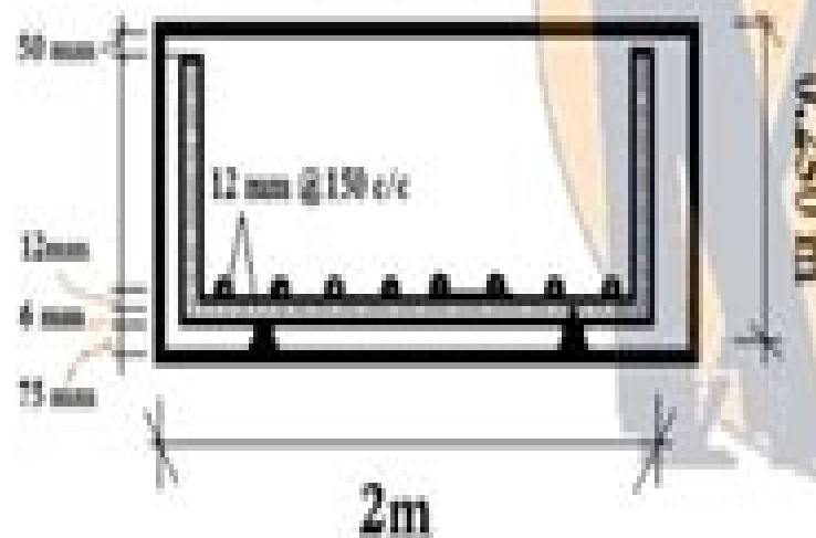
x-Section AA
