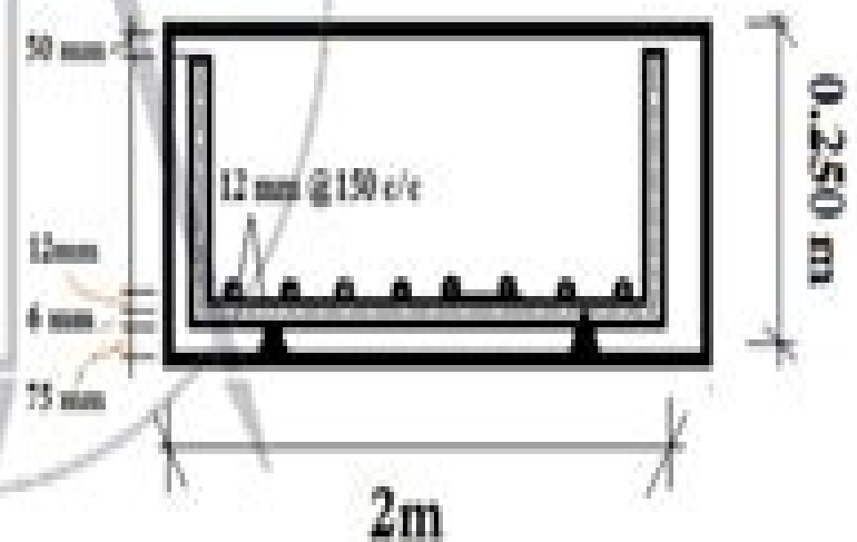
x-Section AA
