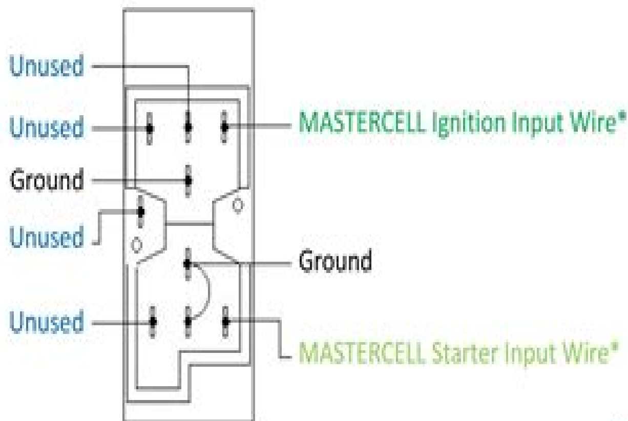
1969-94 Chevrolet / Pontiac Ignition Switch
