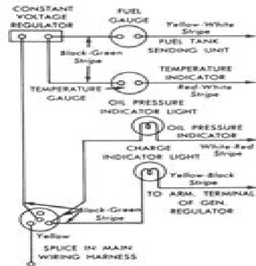
Instrument Gauge Circuit .. 1961-62
