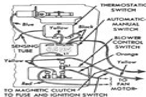
Thermostatic Switch
