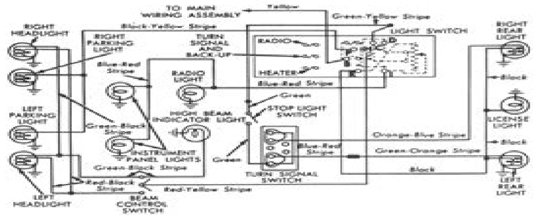
Exterior & Instrument Lamp Circuits .. 1961-62
