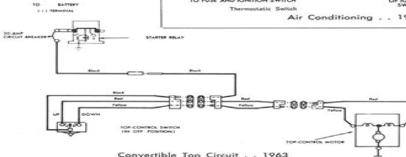
Convertible Top Circuit .. 1963
