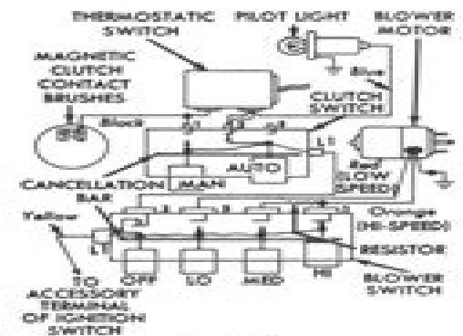
Electrical Control
