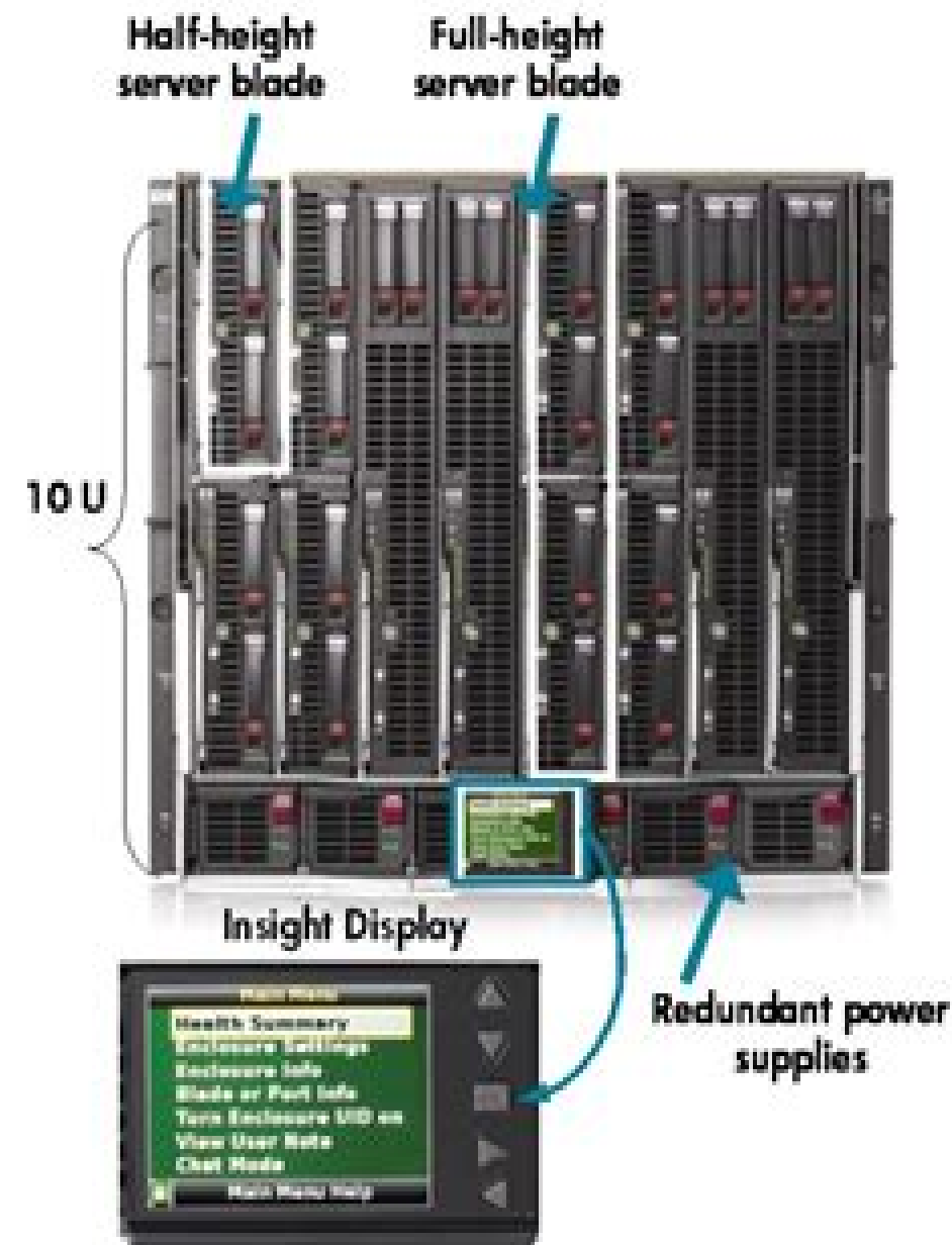
c7000 enclosure - front
