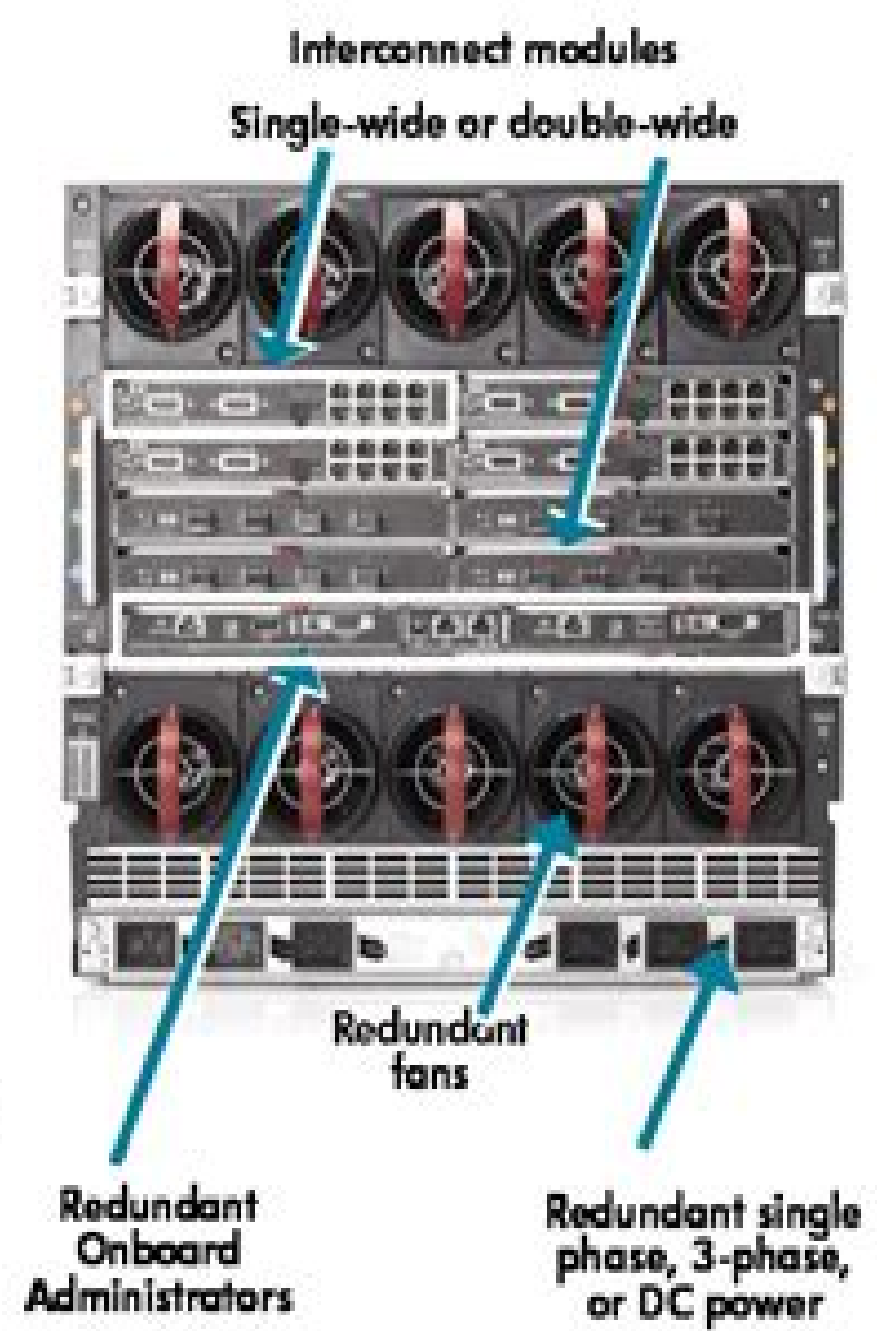
c7000 enclosure - back
