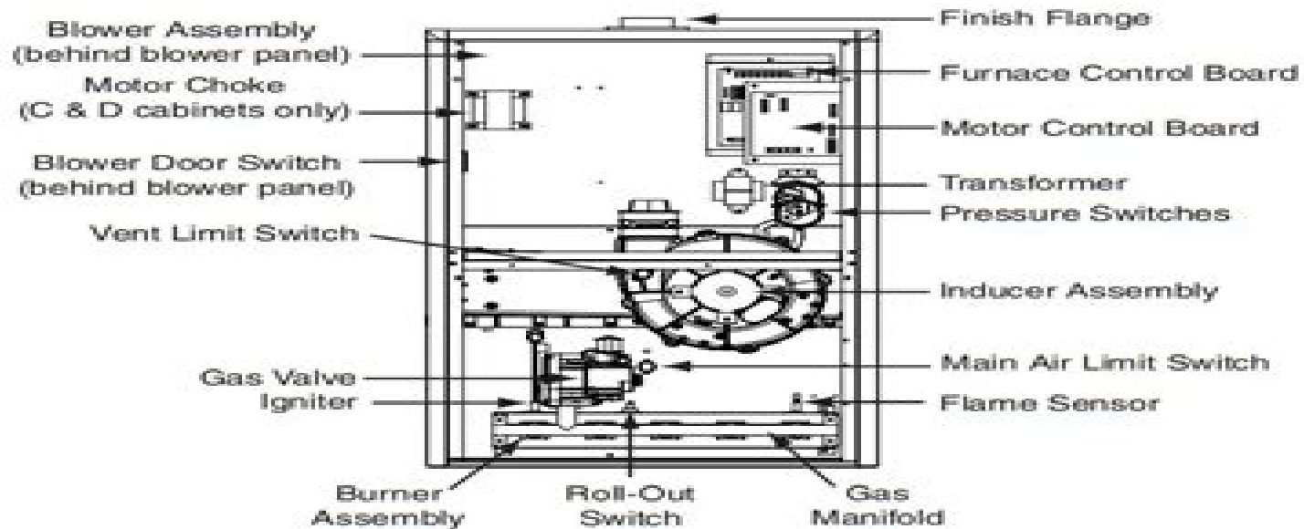
Downflow Gas Furnace Components
