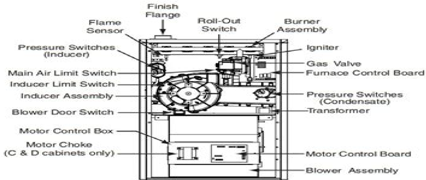
Upflow/Horizontal Gas Furnace Components
