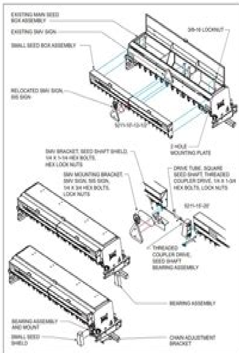
Figure 2-6: Small Seed Assembly Overview (10-12' Drill Shows)
