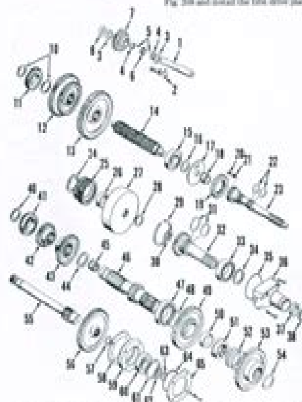
Fig. 203—Exploded view of input shaft, gear and related components used in Multi-Range transmission
