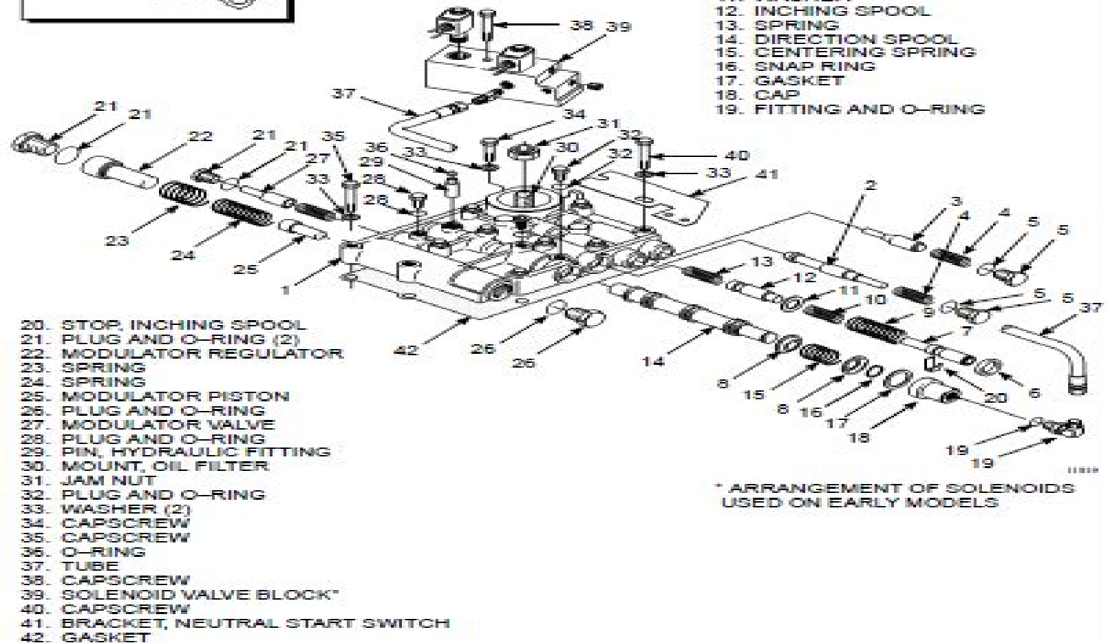
FIGURE 10. CONTROL VALVE, MONOTROL ONLY
